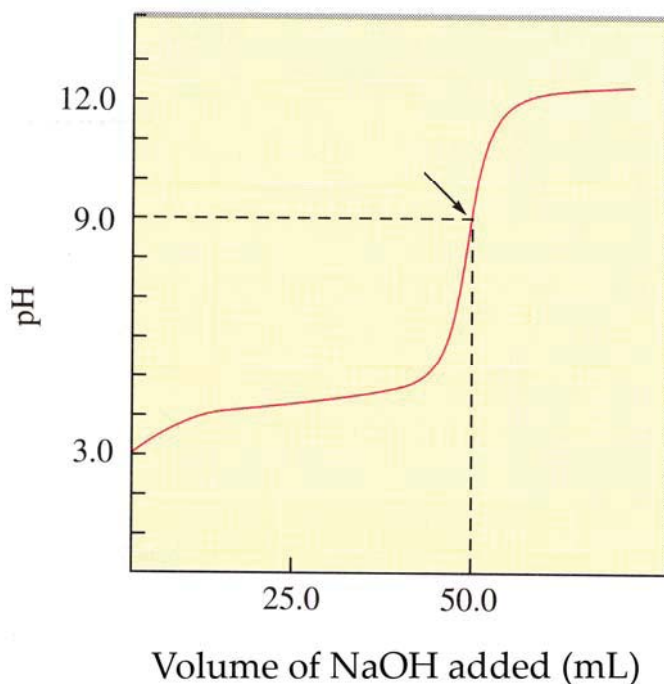
Figure 5- 2: Titration curve
