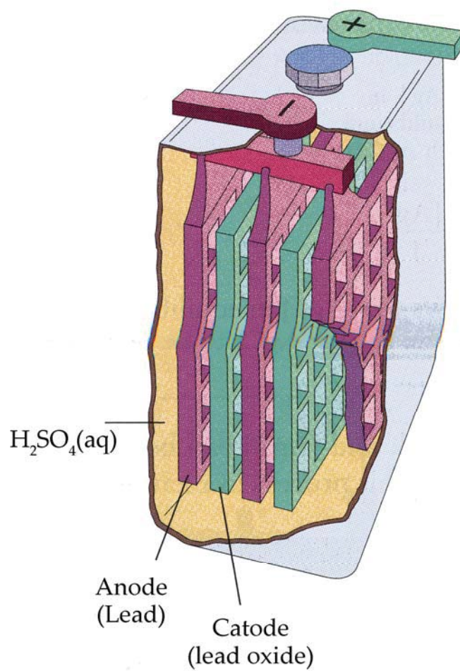
Figure 6- 6: The lead battery The set-up in a lead battery.
